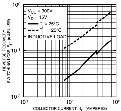
REVERSE RECOVERY SWITCHING LOSS VS. COLLECTOR CURRENT (TYPICAL - INVERTER PART)
