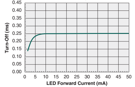
Typical Turn-Off Time vs. LED Forward Current ( I_L=1A_{DC} )
