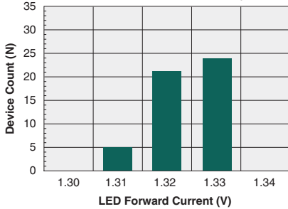
Typical LED Forward Voltage Drop (N=50, I_F=10\text{mA} , I_L=1A_{DC} )
