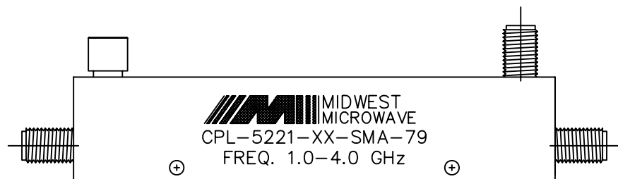
BACKSIDE MARKING
