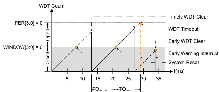
Figure 24-3. Window-Mode Operation
