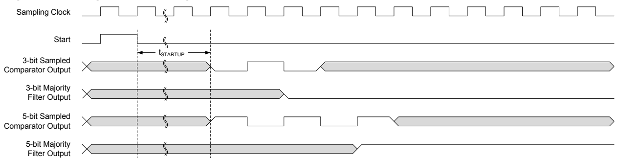
Figure 41-8. Single-Shot Filtering
