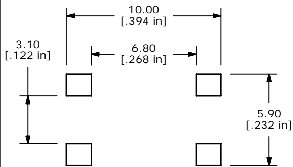
P.C.B MOUNTING
