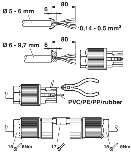
Functional drawing
