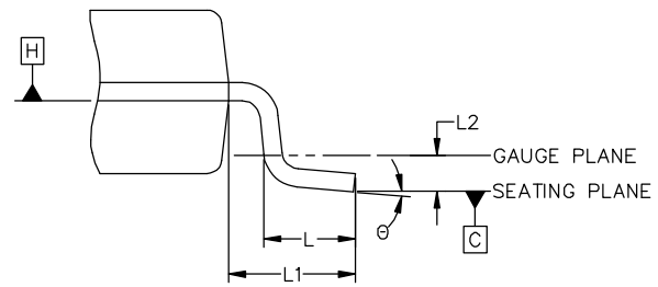
VIEW C
