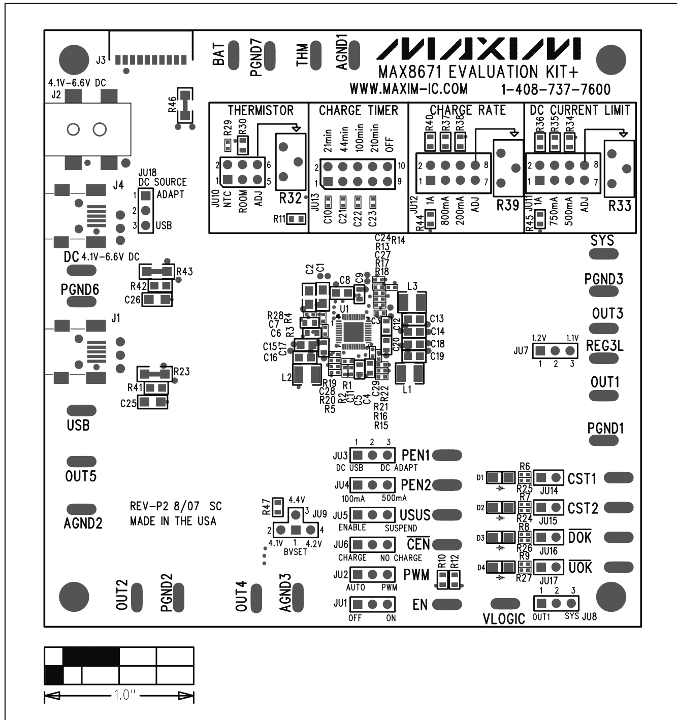
Figure 3. MAX8671 EV Kit Component Placement
