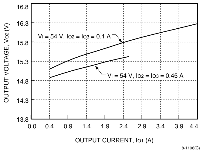
Figure 8. CW025ACL-M Typical Cross Regulation with Respect to I_{o1}
