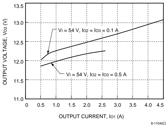
Figure 6. CW025ABK-M Typical Cross Regulation with Respect to I_{o1}
