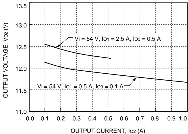
Figure 5. CW025ABK-M Typical Load Regulation
