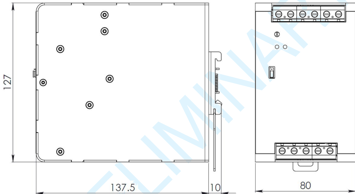
Figure 1. Mechanical Drawing
